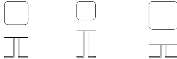
7EL107 Tavolino in metallo Metal coffee table 7EL204 Top marmo/Marble top L50 P50 H43
