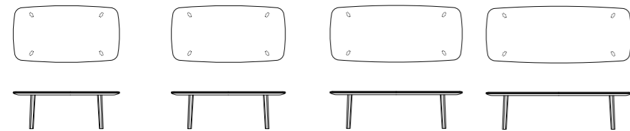
7AND103 Top in marmo / Marble top Base in legno / Wooden base L205 P100 H71,5 7AND102 Top in marmo / Marble top Base in legno / Wooden base L220 P100 H71,5 7AND101 Top in marmo / Marble top Base in legno / Wooden base L255 P110 H71,5 7AND104 Top in marmo / Marble top Base in legno / Wooden base L280 P110 H71,5
