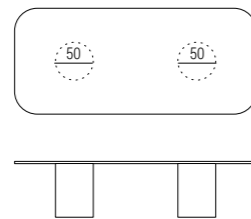
7ART306 Top in marmo/Marble top 7ART316 Top in vetro/Glass top 7ART326 Top in legno/Wooden top L310 P140 H74
