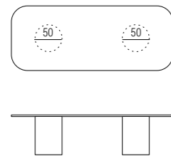
7ART305 Top in marmo/Marble top 7ART315 Top in vetro/Glass top 7ART325 Top in legno/Wooden top L320 P120 H74
