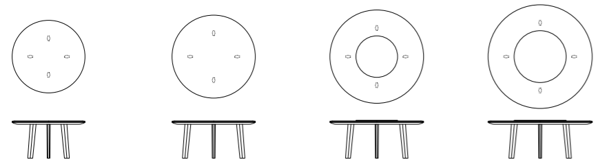
7AND109 Top in marmo / Marble top Base in legno / Wooden base ø140 H71,5 7AND110 Top in marmo / Marble top Base in legno / Wooden base ø160 H71,5 7AND111 Top in marmo / Marble top Base in legno / Wooden base ø180 H71,5 7AND112 Top in marmo / Marble top Base in legno / Wooden base ø200 H71,5
